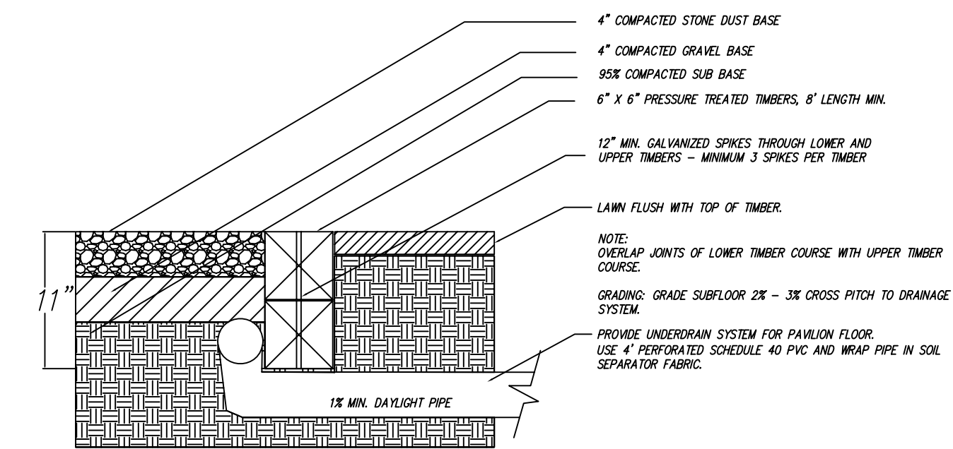
PAVILION OPTIONAL FLOOR DETAIL
